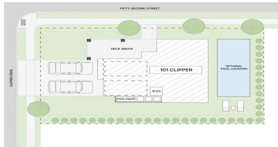
PLOT PLAN
