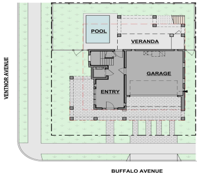
1 PLOT PLAN
