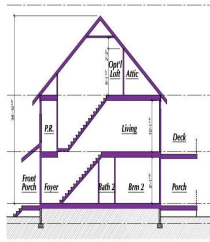
SECTION @ FOYER
