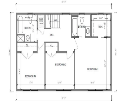
2ND FLOOR PLAN (#23036)
