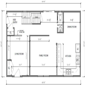
1ST FLOOR PLAN (#23036)
