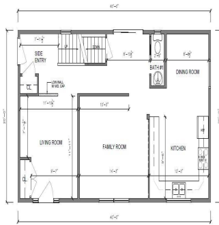
1ST FLOOR PLAN (#23036)
