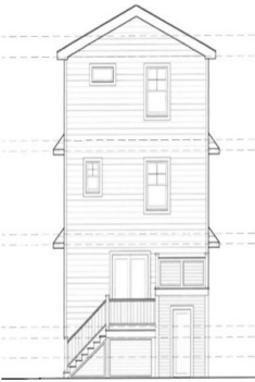
REAR ELEVATION
