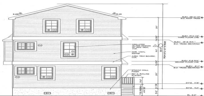
2 REAR ELEVATION
